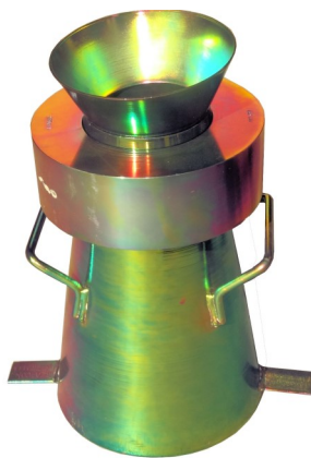
Slump Cone, Filling and Weighted Collar
