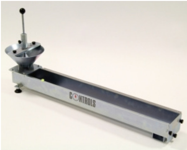
Flow test apparatus for grouts
