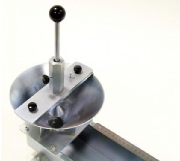
Flow test apparatus: detail of the funnel
