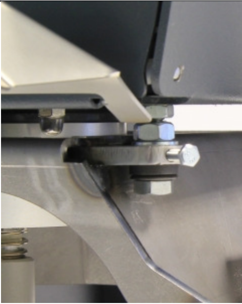
65-L0512 - Detail of the 3-points bowl supporting system allowing precise adjustment of the gap between bowl and beater
