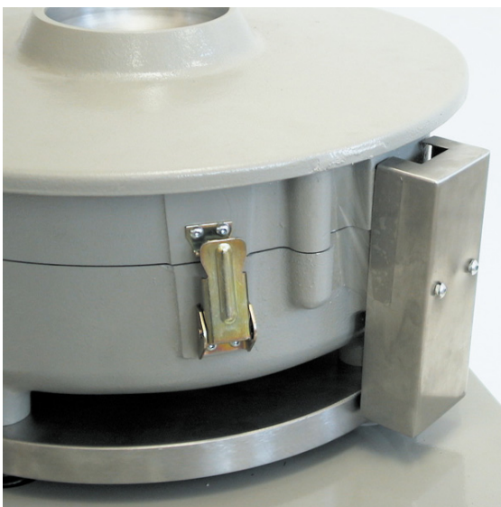
Detail of 75-B2210 UP1 Safety device
