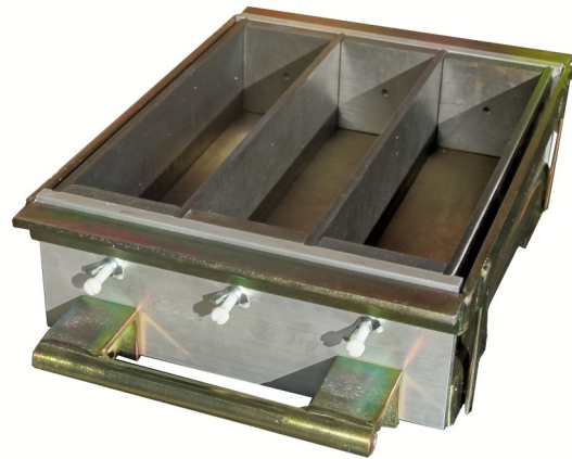
Mould with Handle and Clamping device fitted in position
