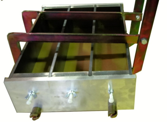
Drying/Shrinkage Mould Lifting Device in operation
