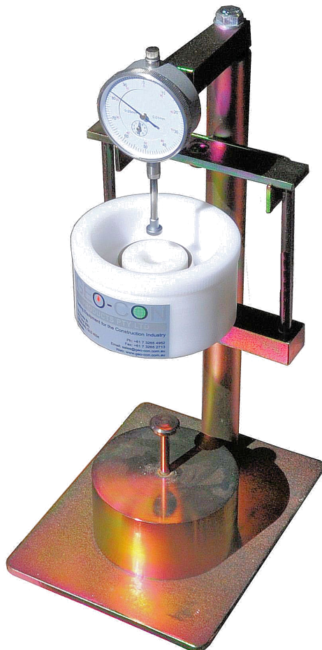
Single Shrink/Swell set-up
