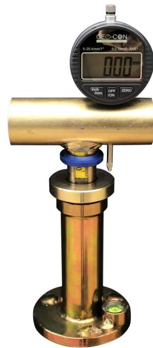
Digital Dial Gauge in use
